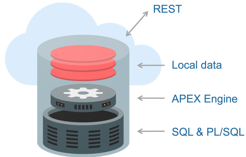
Oracle Database
